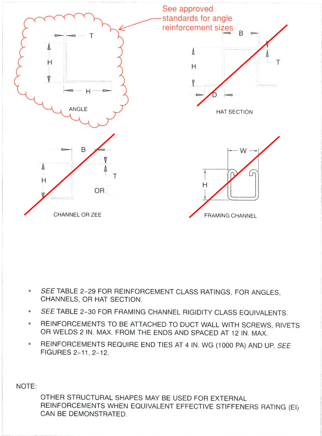
FIGURE 2-3 RECTANGULAR DUCT EXTERNAL REINFORCEMENTS
